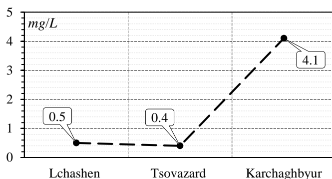
Fig. 5. DO content in Lake Sevan in July 2019.
